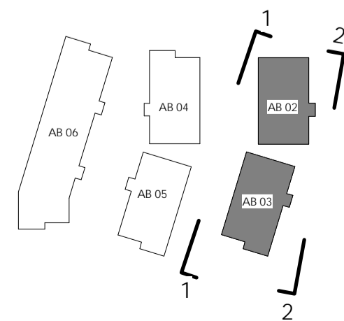
APARTMENT BLOCKS 02-06 SITE KEY PLAN
