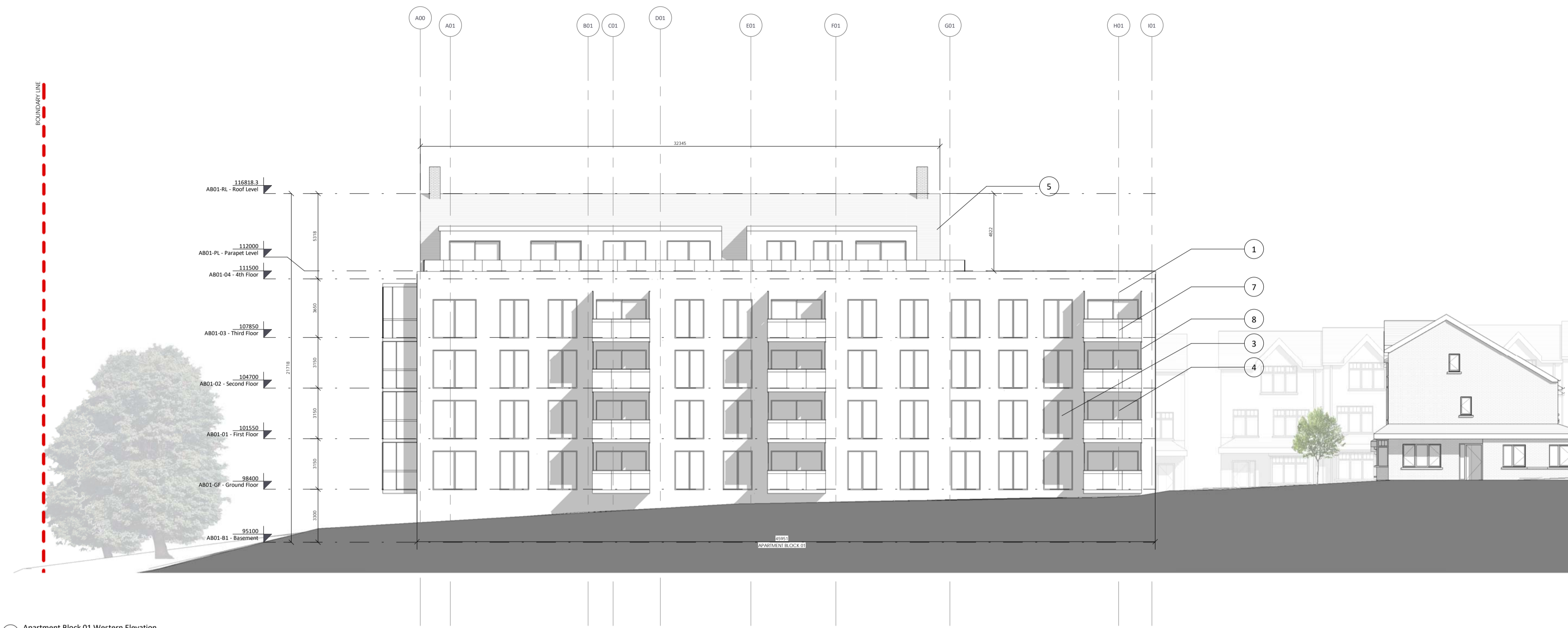
1 Apartment Block 01 Western Elevation 1:200
