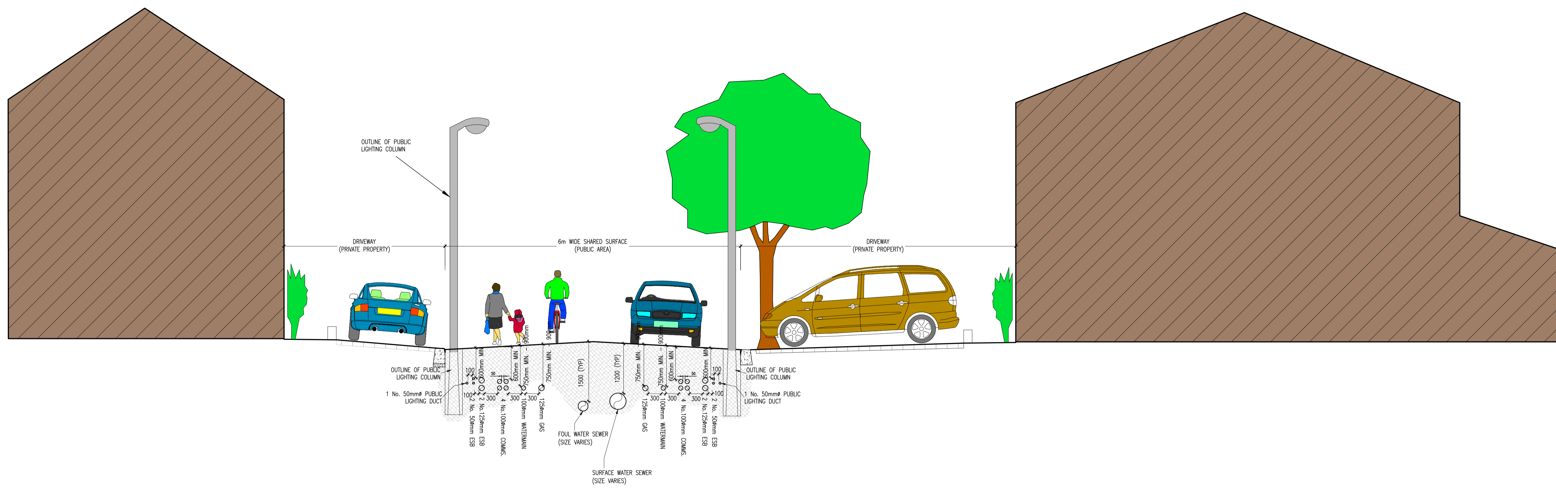
TYPICAL CROSS SECTION SHOWING SERVICES UNDER SHARED SURFACE AREAS (SCALE 1:50)
