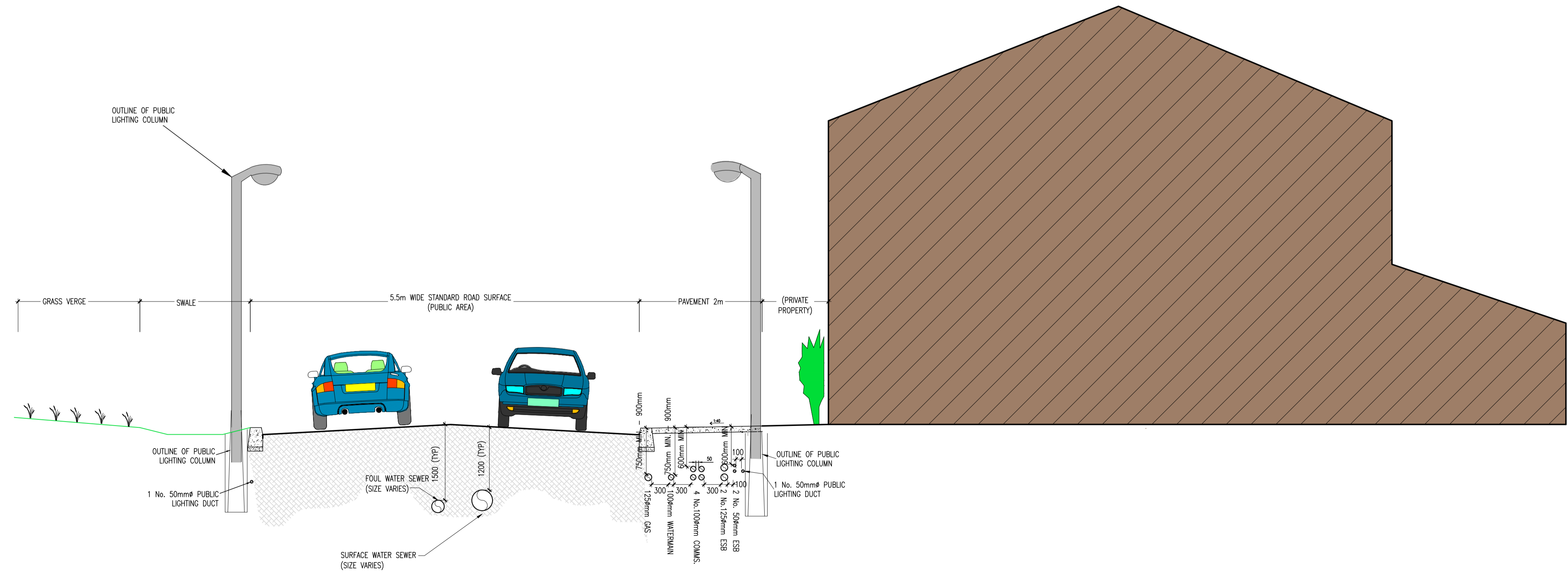
TYPICAL CROSS SECTION SHOWING SERVICES UNDER SHARED STANDARD ROAD (SCALE 1:50)
