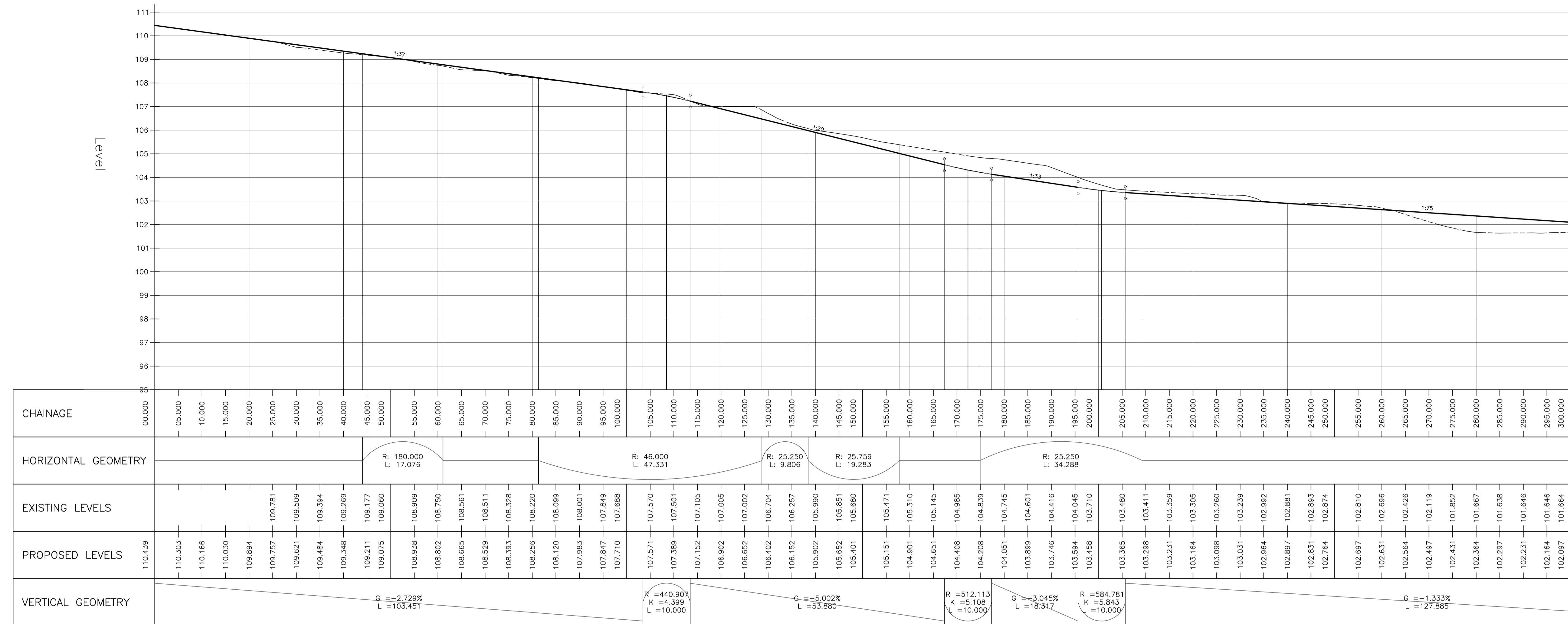
ROAD 1 – LONGSECTION SCALE: H 1:500, V 1:100.
