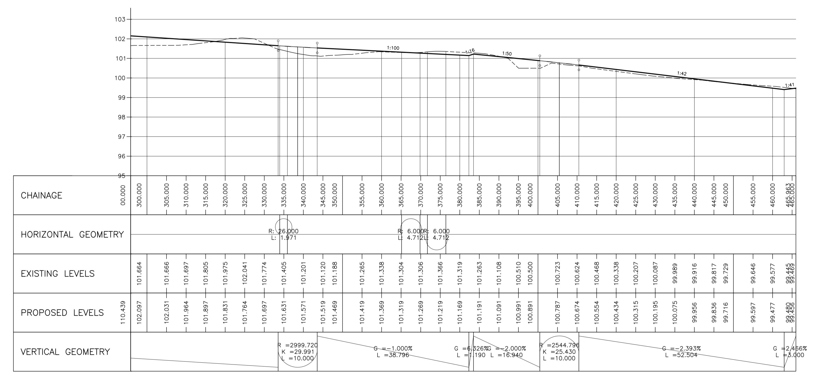
ROAD 1 – LONGSECTION SCALE: H 1:500, V 1:100.
